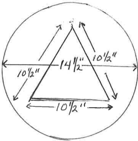
BASE OF ANTENNA
