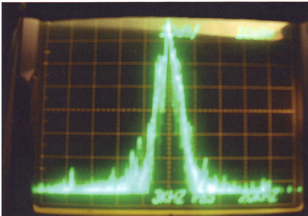
Occupied Bandwidth 10db/div 20khz/div
