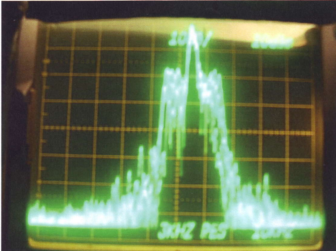
Occupied Bandwidth 10db/div 10khz/div
